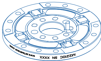
DRAWING IN THIRD ANGLE PROJECTION
